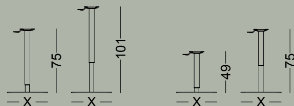
Con piastra standard 170x170 With standard plate 170x170
