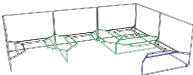
Cinque posti Five seats
